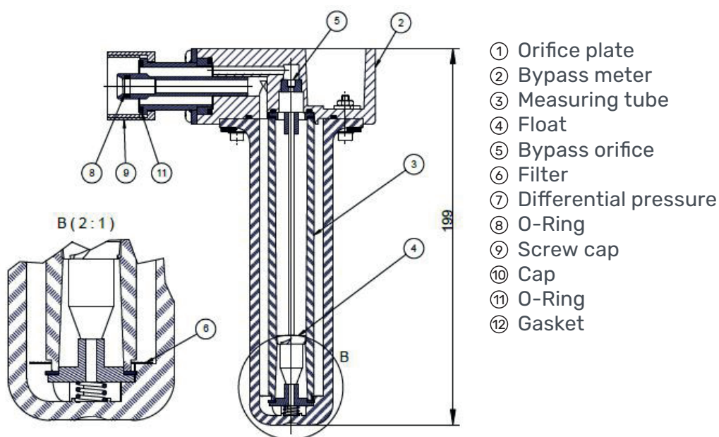
Fig. 2: Position drawing bypass orifice
