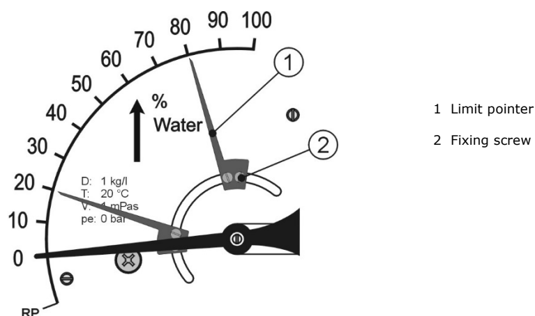
Fig. 2 Adjustment of the switching point (limit switch)
