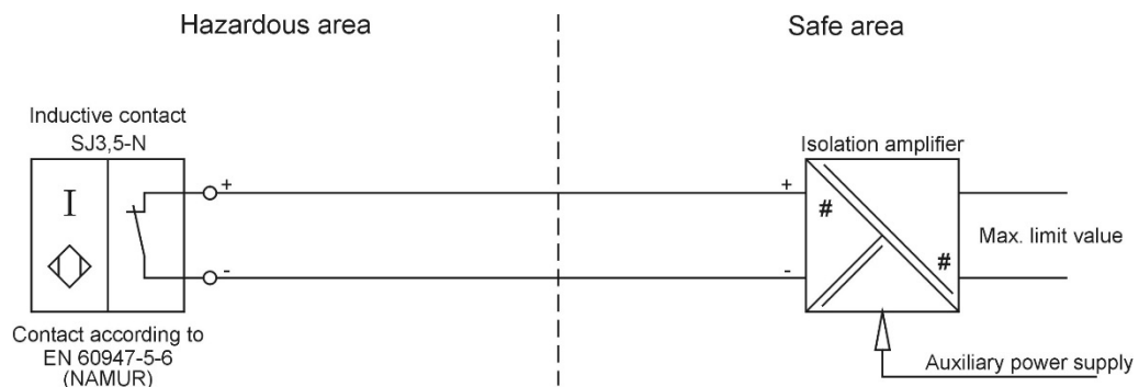
Fig. 13 Connection diagram for RE 250 with one limit switch
