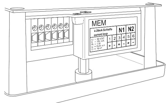
Fig. 16 Terminals (with add. digital
