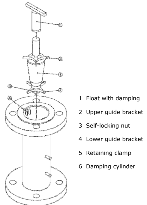
Fig. 3 Replacing float damping
