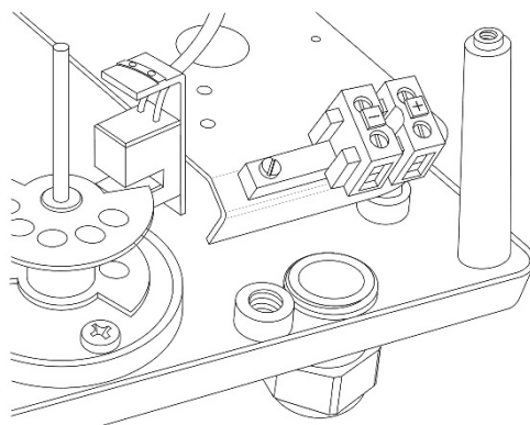
Fig. 11 Terminals (one limit switch)
