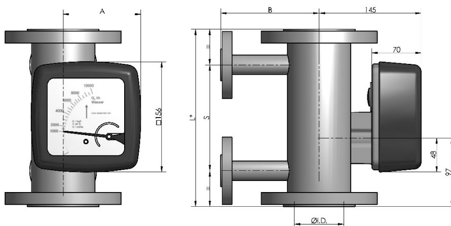
Heating shield version
