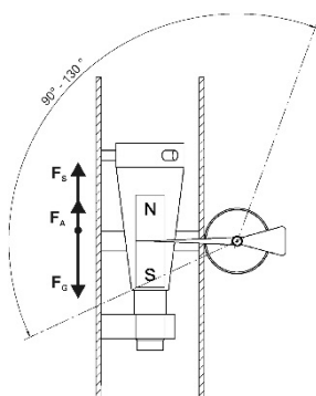
Fig. 1 Operating principle of the RE 250
