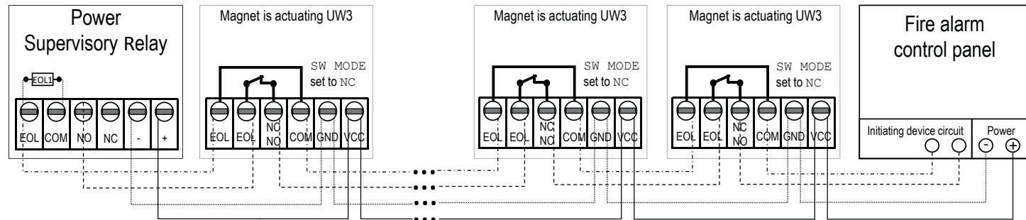
Fig. 3: Series wiring configuration*
