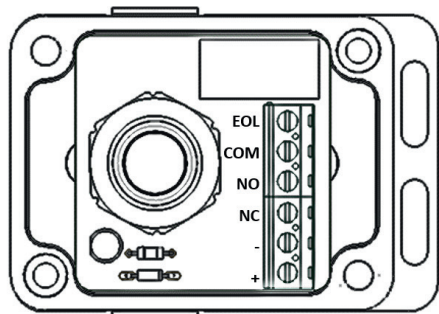
Fig. 2: Terminal and internals
