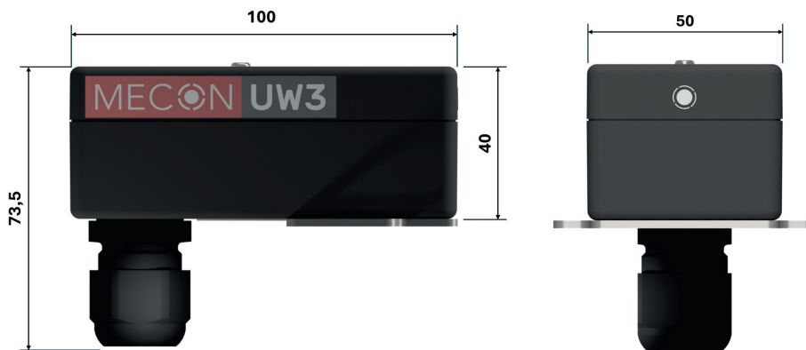
Fig. 1: Dimensions UW3 (mm)
