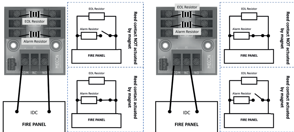
Fig. 2: Example wiring configuration
