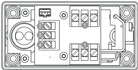
Fig. 1: Terminal and internals
