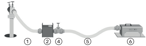
Fig. 5: Setup without turbidity sensor
