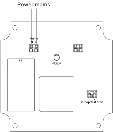
Fig. 2: Wiring diagram Key Switch Group
