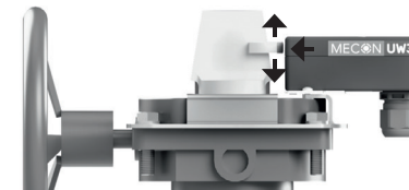
Fig. 6: Final positioning of the magnet holder
