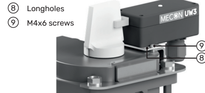
Fig. 4: Correct alignment of all components
