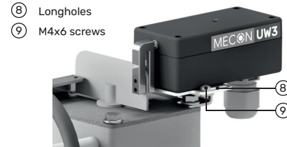
Fig. 4: Correct alignment of all components
