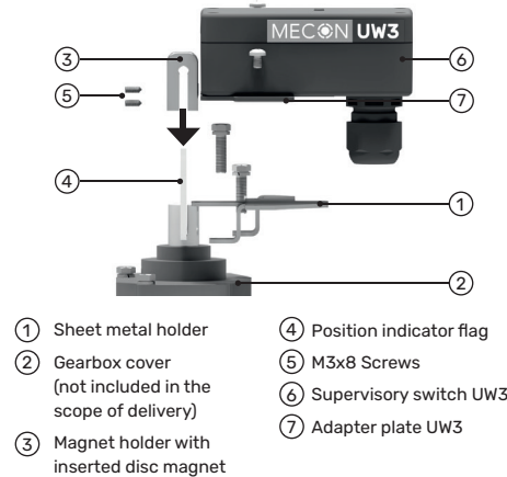
Fig. 3: Components and assembly
