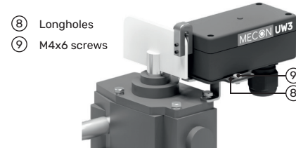
Fig. 4: Correct alignment of all components
