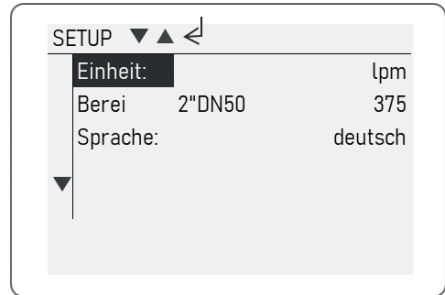
Abb. 7: Display Setup-Menü
