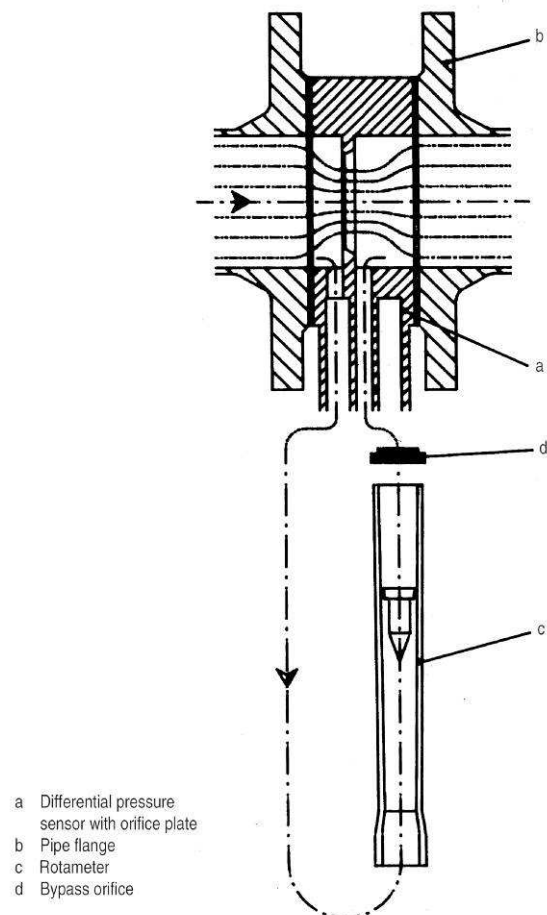
Fig. 2 Measuring principle
