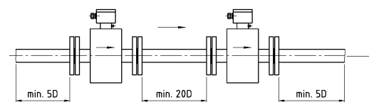
Fig. 5 Installation between tees, valves and pumps
